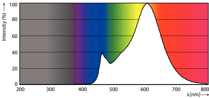
LED Bulb CLA 8-75W E27 A60 Clear 827 ND
