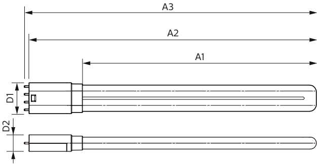
PLED 230V 16-36W 2100lm 3000K 2G11
