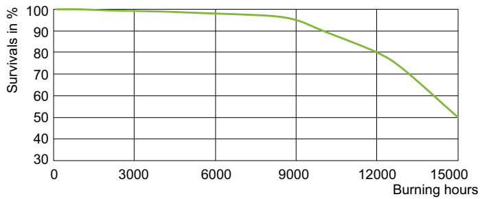
CDM-R Elite 70 W Life Expectancy /942 E27 PAR30L
