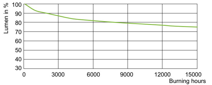
CDM-R Elite 70 W Lumen Maintenance /942 E27 PAR30L
