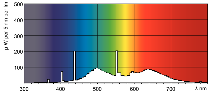
LDPO_TL-D9HCR_950-Spectral power distribution Colour
