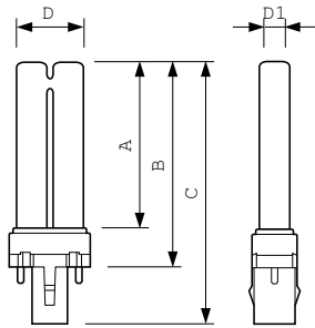
TUV PL-S 9W/2P
