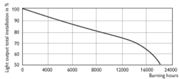
SON-T Comfort
