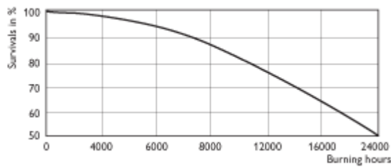
SON-T Comfort
