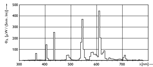
Typical Spectral energy distribution of QL 85W 3000K.
