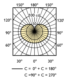
Typical light distribution of QL 85W
