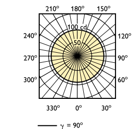
Typical light distribution of QL 85W, Azimuth angle
