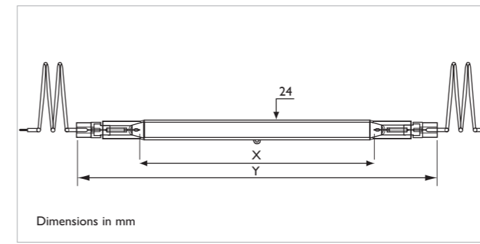
Philips HOK 10/120L, HOK 15/120L, HOK 20/120L, HOK 25/120L
