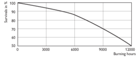
MASTER MHN-LA 2000W/842/956 400V
