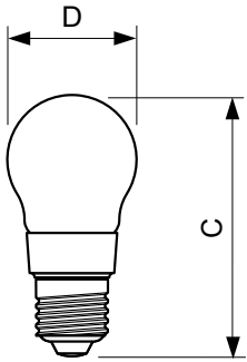
filament 2.5W-25W 250lm NAD 2700K E27D
