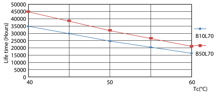
LEDtube_30K_4060_LifetimeVsTc-LED
