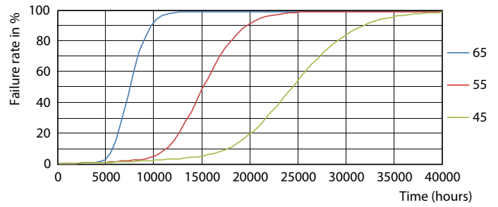
LEDtube 15K 4565 FailureRate-LED
