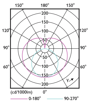
LEDtube ECO RCA 18W G13 1650lm-LDD
