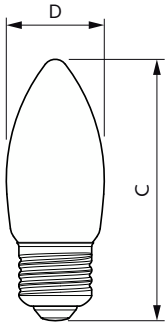
LEDClassic 4.5W B11 E27 850 CL ND 3CT/10
