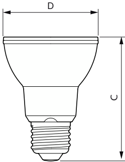
5.5PAR20/LED/F40/940/DIM/G/T20 6/1FB
