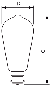
MASTER VLE EDBulbDT5.9-60W B22 927 ST64CL G
