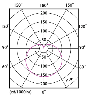
LEDbulb G6 A19 5W E26 950 FR-LDD
