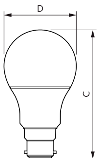
MASTER LEDbulb DT 5.5-40W B22 A60 CL
