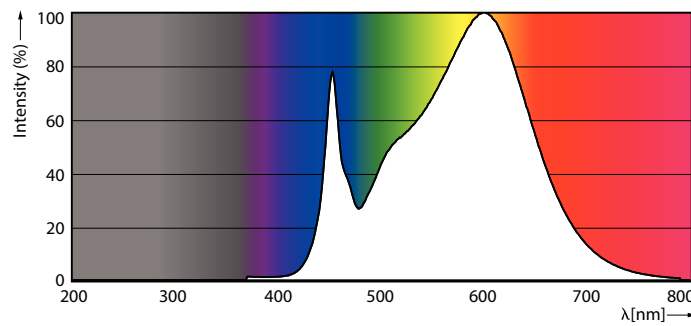
LEDtube MAS 14,5W G13 2000lm 835
