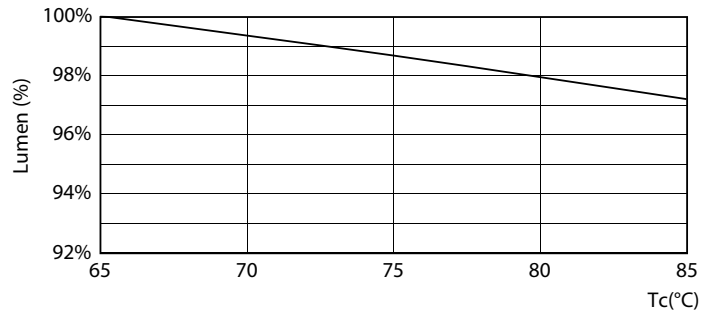
LEDtube PLC 11W 15K 1 LumenVsTc
