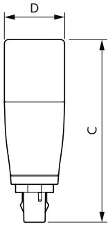
LED PLC 11W 830 2P G24D
