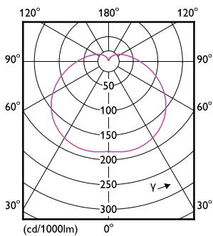
LEDTForce Core GC 40W Tshape E27-LDD
