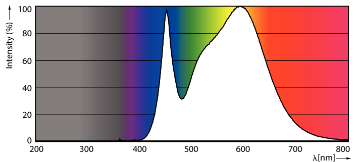
LEDTForce Core GC 40W Tshape E27 840-POC
