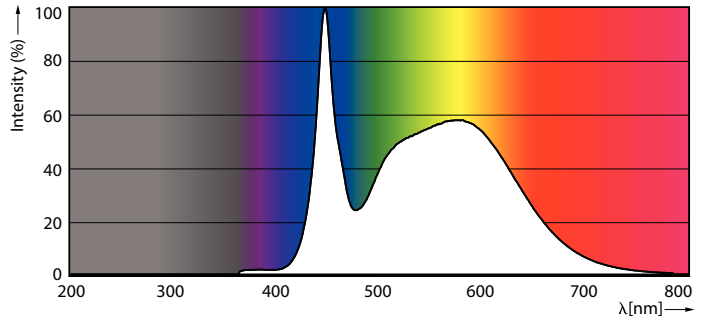
LEDTForce 40W WallPack EX39 850
