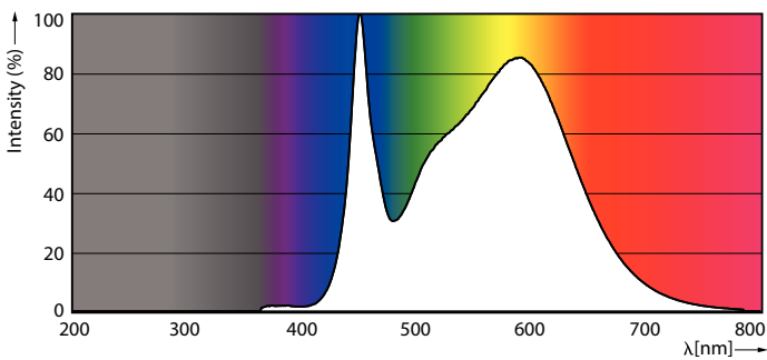
LEDTForce 40W WallPack EX39 840
