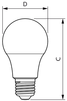
EcoHome LEDBulb 10W E27 3000KLV 1PF/12NL
