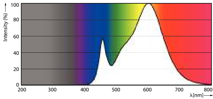
LEDbulb ECO 10W A19 E27 830 FR
