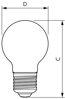
LEDClassic4.5W G16.5 E27 827 CLND 3CT/10
