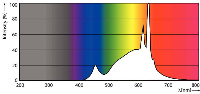
LEDbulb 8,8W A19 E26 927 FR
