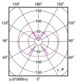
LEDbulb CLA A19 8,5W E26 922 927 FR-LDD
