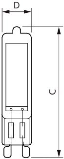
LEDcapsule 40W G9 827 120V ND
