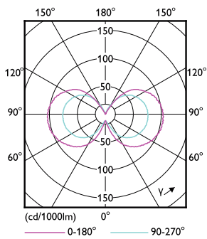
LEDcapsule 4W G9 827
