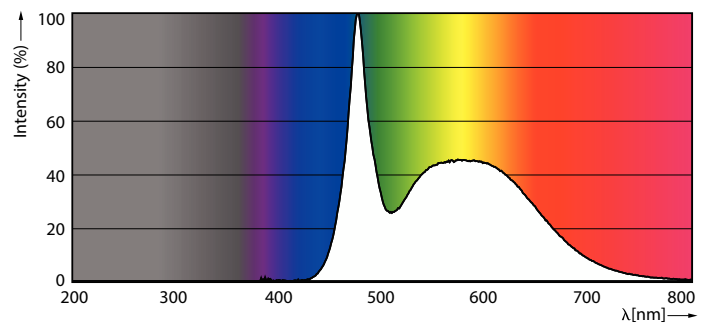
LEDbulb ESS 14W A19 E27 865 FR
