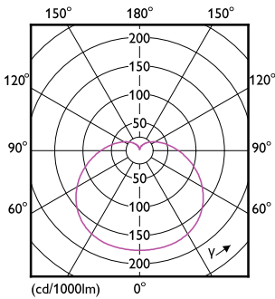
LEDbulb Ecohome A60 14W E27 1150lm 830 FR
