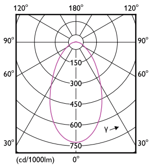
LEDTForce HB 140W Others E40 60D
