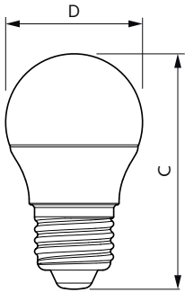
LED candle/luster LEDBulb 4W E27 3000K 100-240VG45 BR
