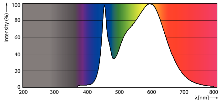
LEDTrueForce HB EX39 200D 840
