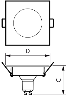
LEDspot50W GU10Kit_S 865 100-240V 36D PF
