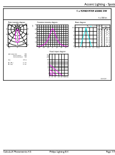
LEDspots ESS K 5W PAR16 G10 865 36D
