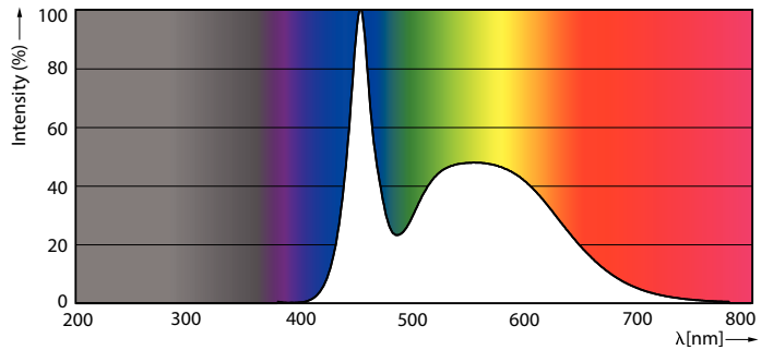
LEDspots ESS K 5W PAR16 G10 865 36D
