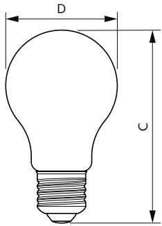
LEDClassic 35W A60 E27 825 100-240V NDBR
