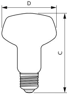
ESS LED 9W E27 2700K 230V R80
