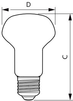
ESS LED 7W E27 6500K 230V R63
