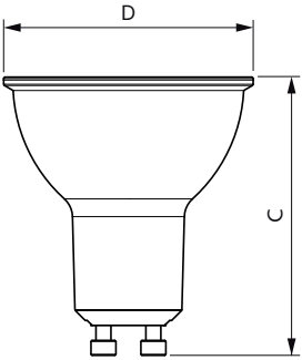
ESSLEDspot 6W 500lm GU10 827 120D ND RCA
