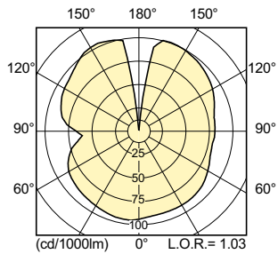
CDO-TT Plus 250W /828 E40 horizontal (HOR) burning
